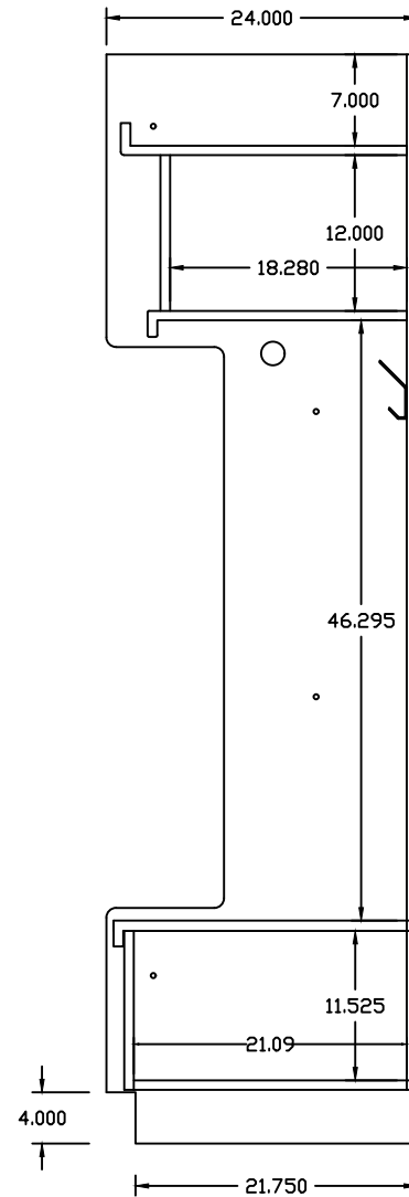
Side View
