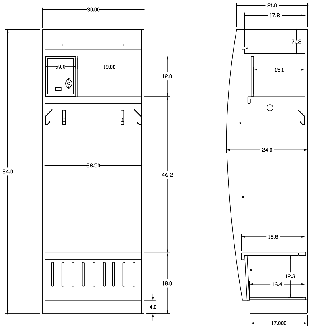
FRONT VIEW
