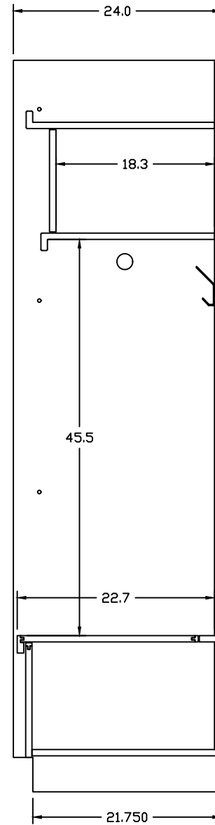
SIDE VIEW
