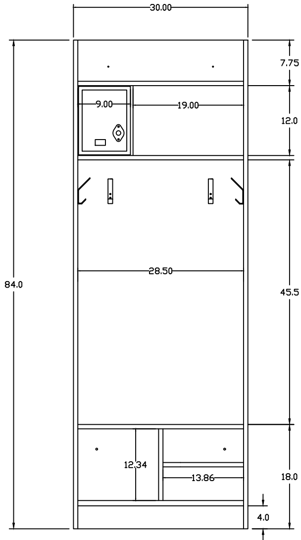
FRONT VIEW
